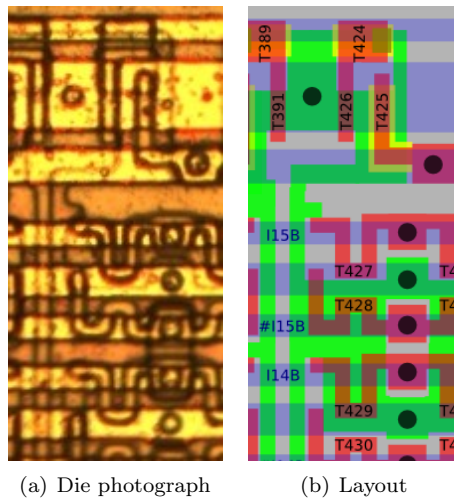
Figure 4.15: A part of the product term array
